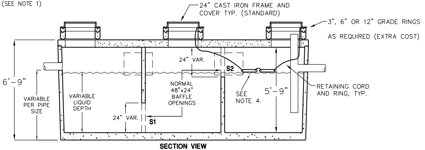
SECTION VIEW
