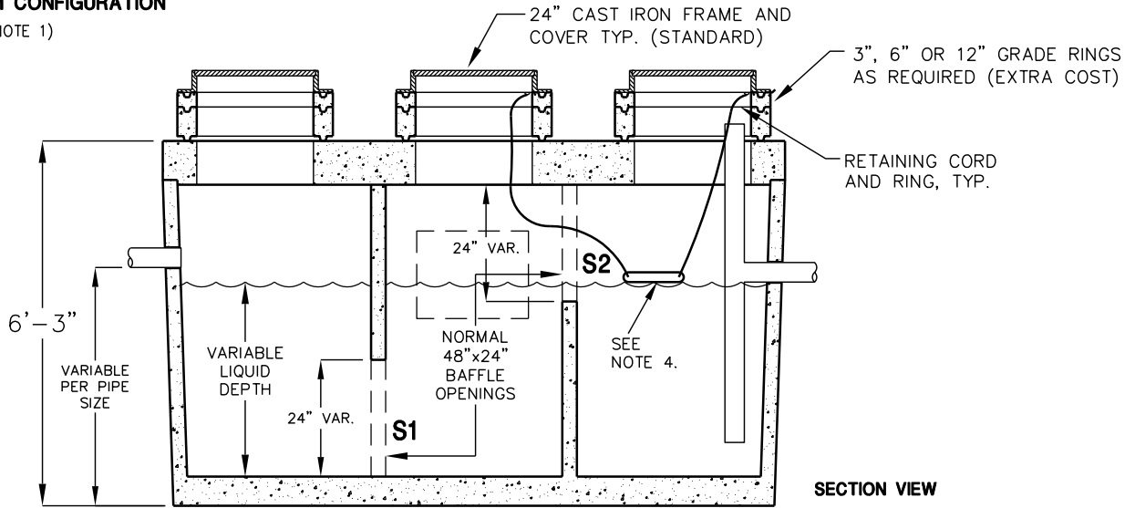
STORMWATER INTERCEPTOR TYPICAL SYSTEM CONFIGURATION (SEE NOTE 1)
