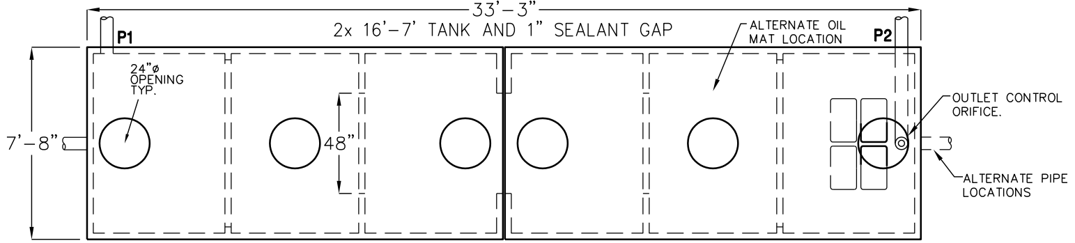
TOP VIEW (COVERS & RISERS REMOVED)
