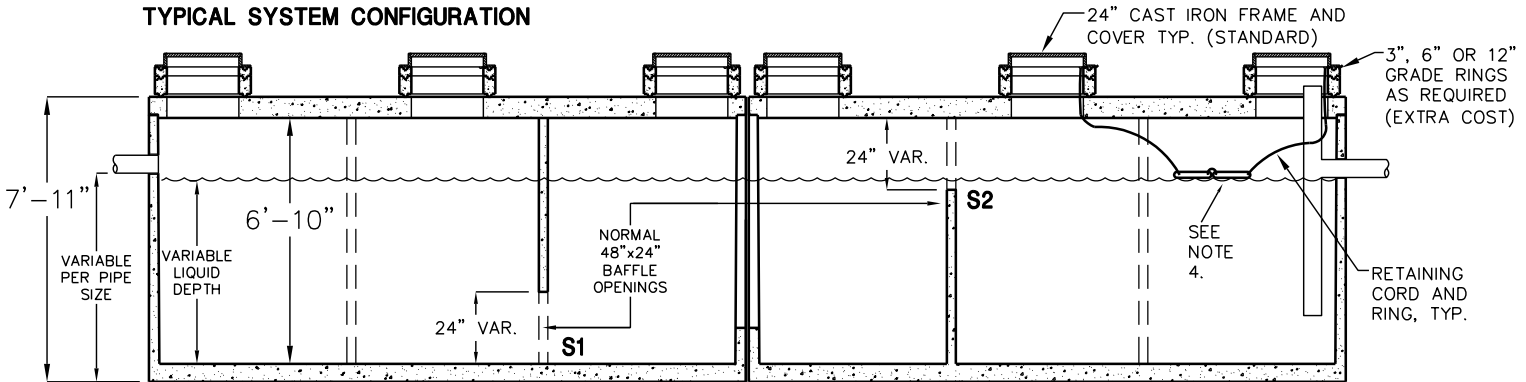
SECTION VIEW
