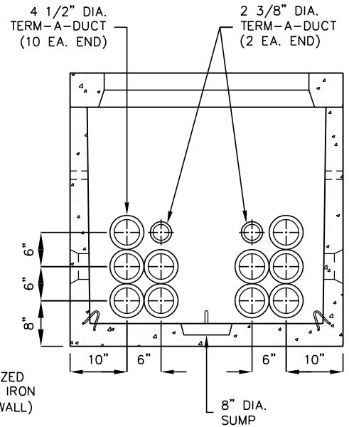
END VIEW (TYP.)
