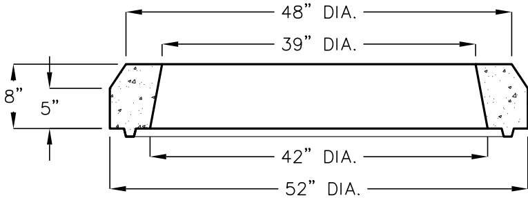
ELEVATION SECTION
